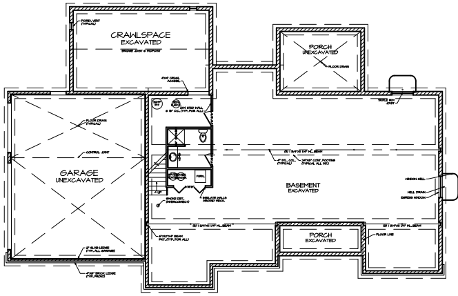
FOUNDATION PLAN A-1
